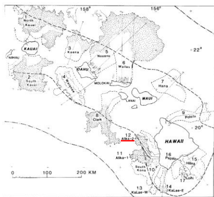
Fig. 3. Map of southeastern Hawaiian Ridge showing major faults bounded by dashed lines identified by number in text and Table 1; compare with Figure 1. Dotted area, hornedocks ground (widely spaced where subside); hatched lines, seeps; thin down-slope directed lines, submarine canyons and their subparallel counterparts; heavy dashed line, axis of the Hawaiian Trench; dash-dotted line, crest of the Hawaiian Arch.
