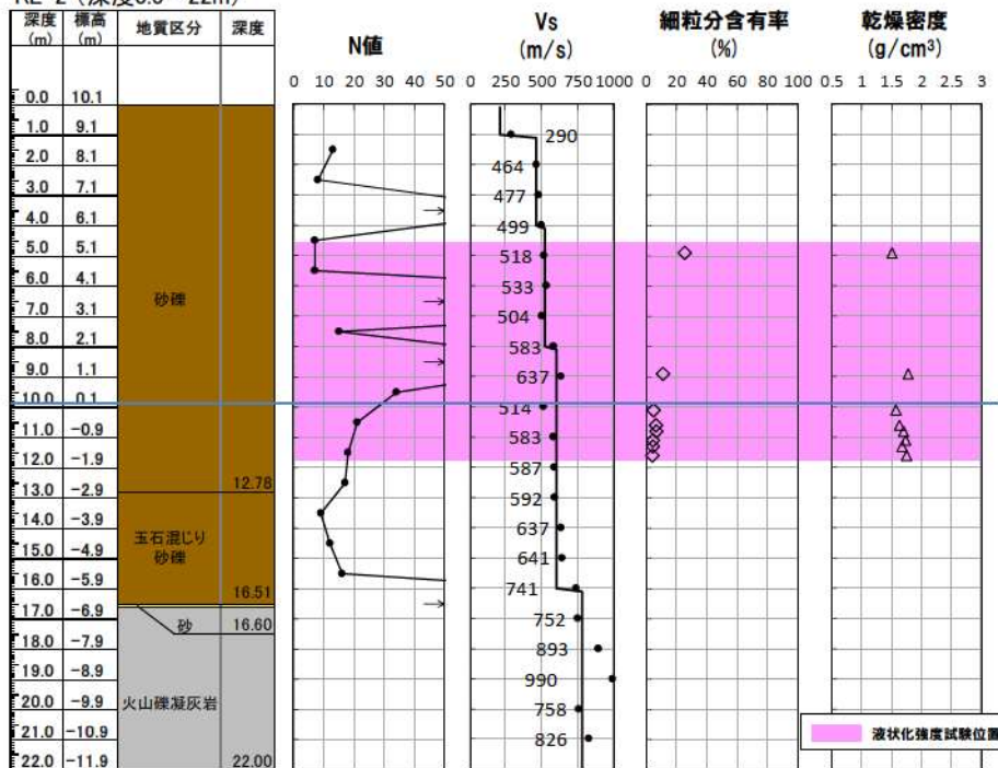
RE-2 (深度0.0~22m)
