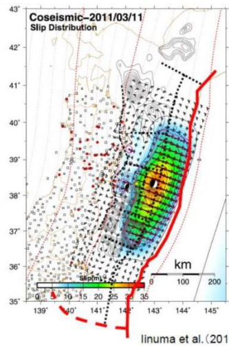
Iinuma et al. (2011)
