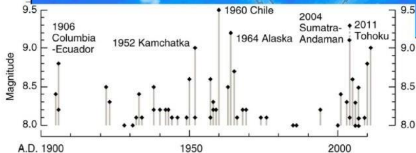
Updated Satake and Atwater (2007, Ann. Rev. Earth Planet. Sci.)
