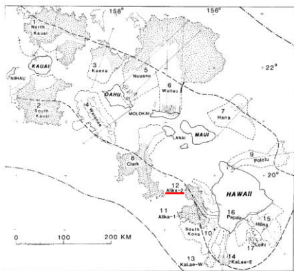
Fig. 3. Map of southeastern Hawaiian Ridge showing major slides bounded by dashed lines identified by number in text and Table 1; compare with Figure 1. Dotted area, hornedocks ground (wavy spaced where subside); hatched lines, scarp; thin down-slope directed lines, submarine canyon and line (subparallel counterparts); heavy dashed line, axis of the Hawaiian Trench; dash-dotted line, crest of the Hawaiian Arch.
