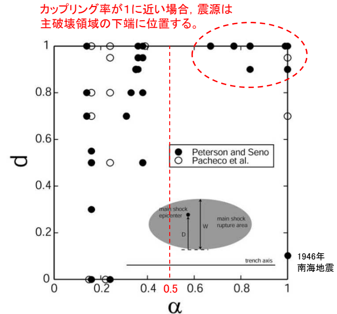
Fig. 1. The relative hypocentral depth d versus the seismic coupling coefficient α obtained for large interplate earthquakes at subduction zones (Table 1). Solid and open circles stand for α values from Peterson and Seno [7] and from Pacheco et al. [15], respectively. When α is estimated to be greater than 1 (Table 1), it is reduced to 1. The relative hypocentral depth d is defined by D / W , where D is the distance from the trenchward edge of the rupture area to the epicenter and W is the width of the rupture area in the direction perpendicular to the trench axis (inset).
