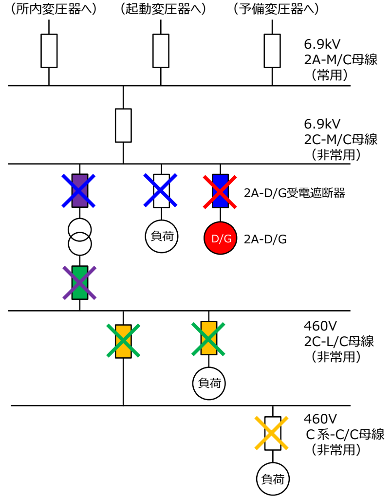
図5 D/G給電
