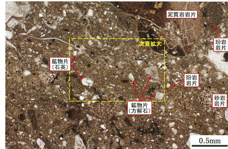
(3) b: 破碎帯[f-161断層]
