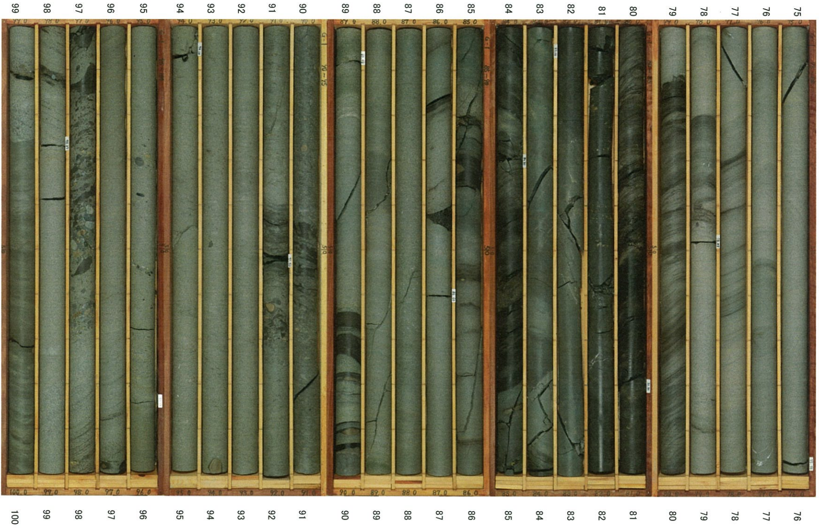
G-1孔 (4/10) 深度75~100m
