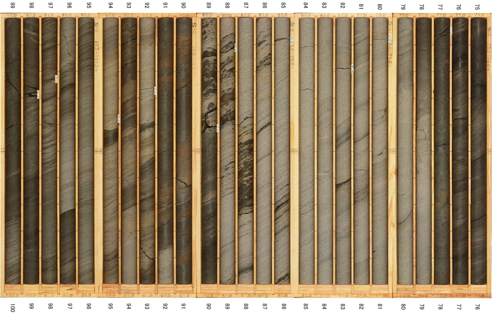
S-5孔 (4/8) 深度75~100m
